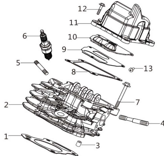
Figure 1 - Overhead Valve
