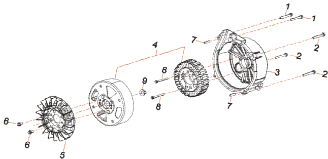
Figure 15 - Rotor/Stator
