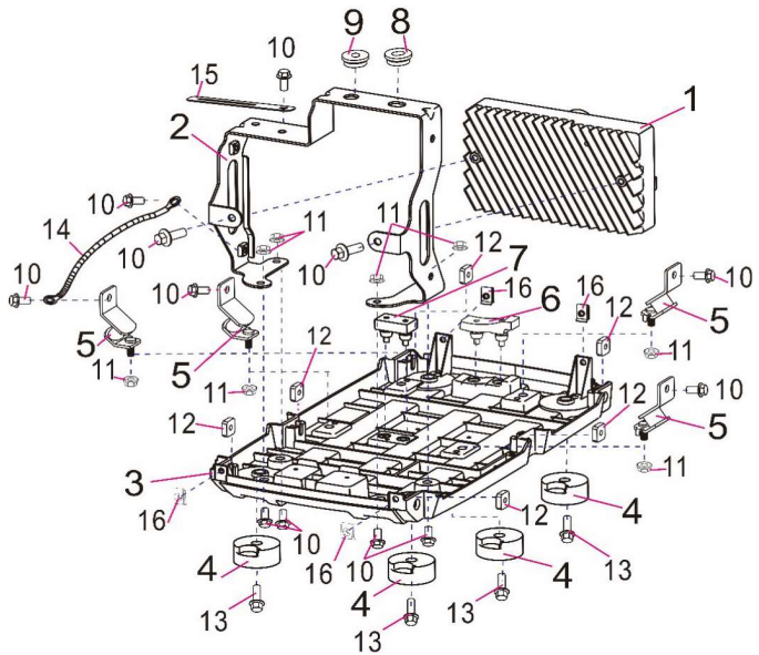
Figure 13 - Baseplate, Inverter
