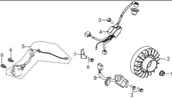
Figure 6 - Flywheel, Impeller, Starter Pulley, Ignition Coil
