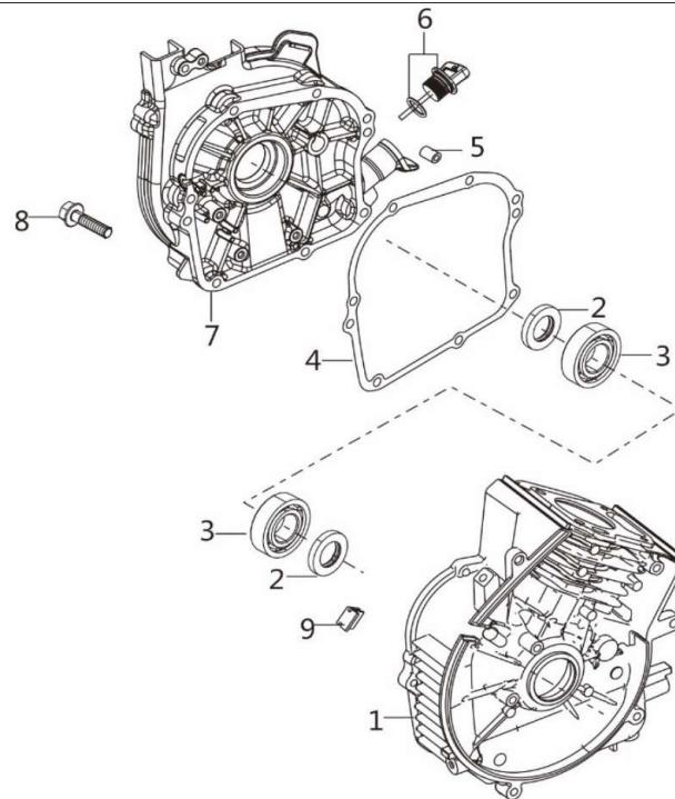
Figure 2 - Crankcase Cover
