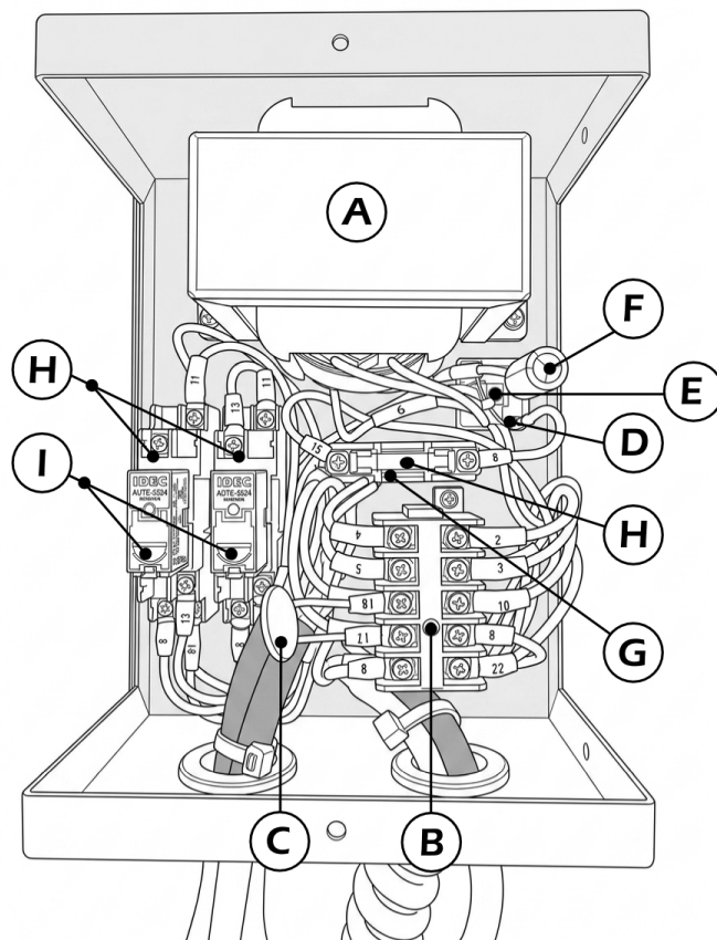
Figure 1 1BR512911B Control Box Assembly
