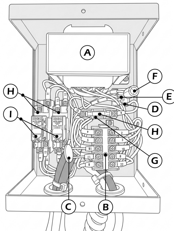
Figure 1 1BR512911B Control Box Assembly
