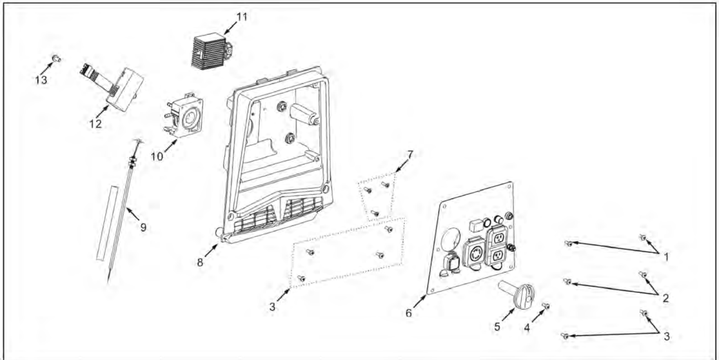
Figure 12 - Control Panel
