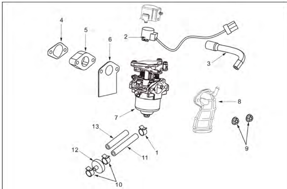
Figure 8 - Carburetor Parts
