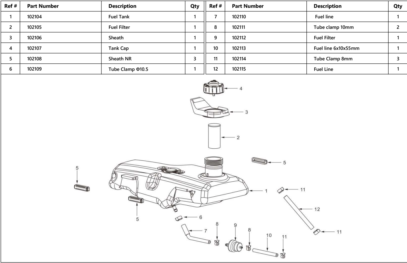
Figure 2 - Fuel Tank
