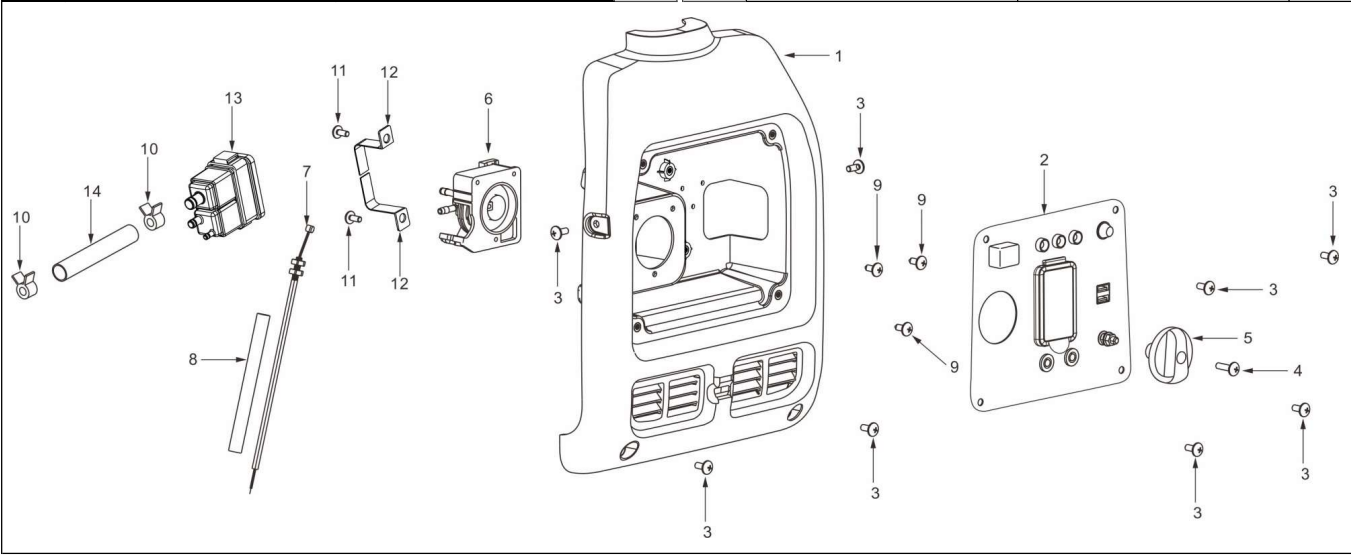
Figure 8 - Engine: Rotor/Stator
