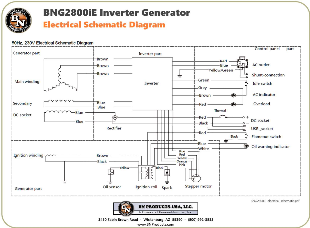
Figure 17 - Electrical Schematic
