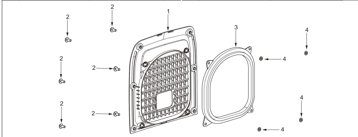
Figure 4 - Left Housing
