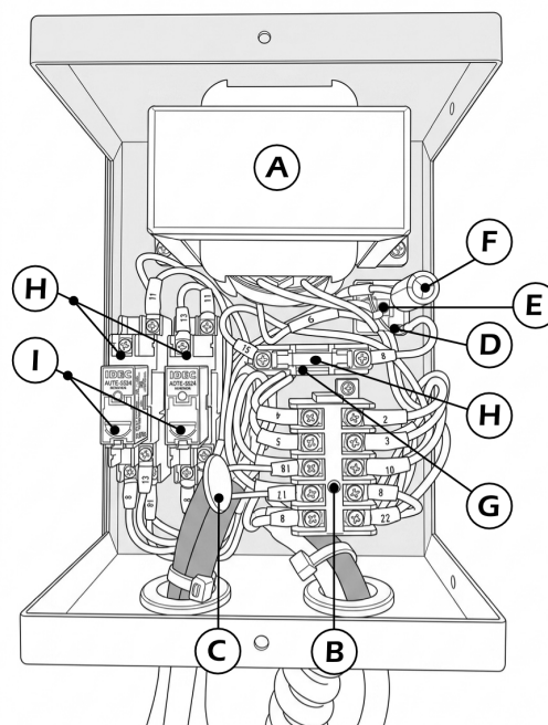
Figure 1 1BR512911B Control Box Assembly
